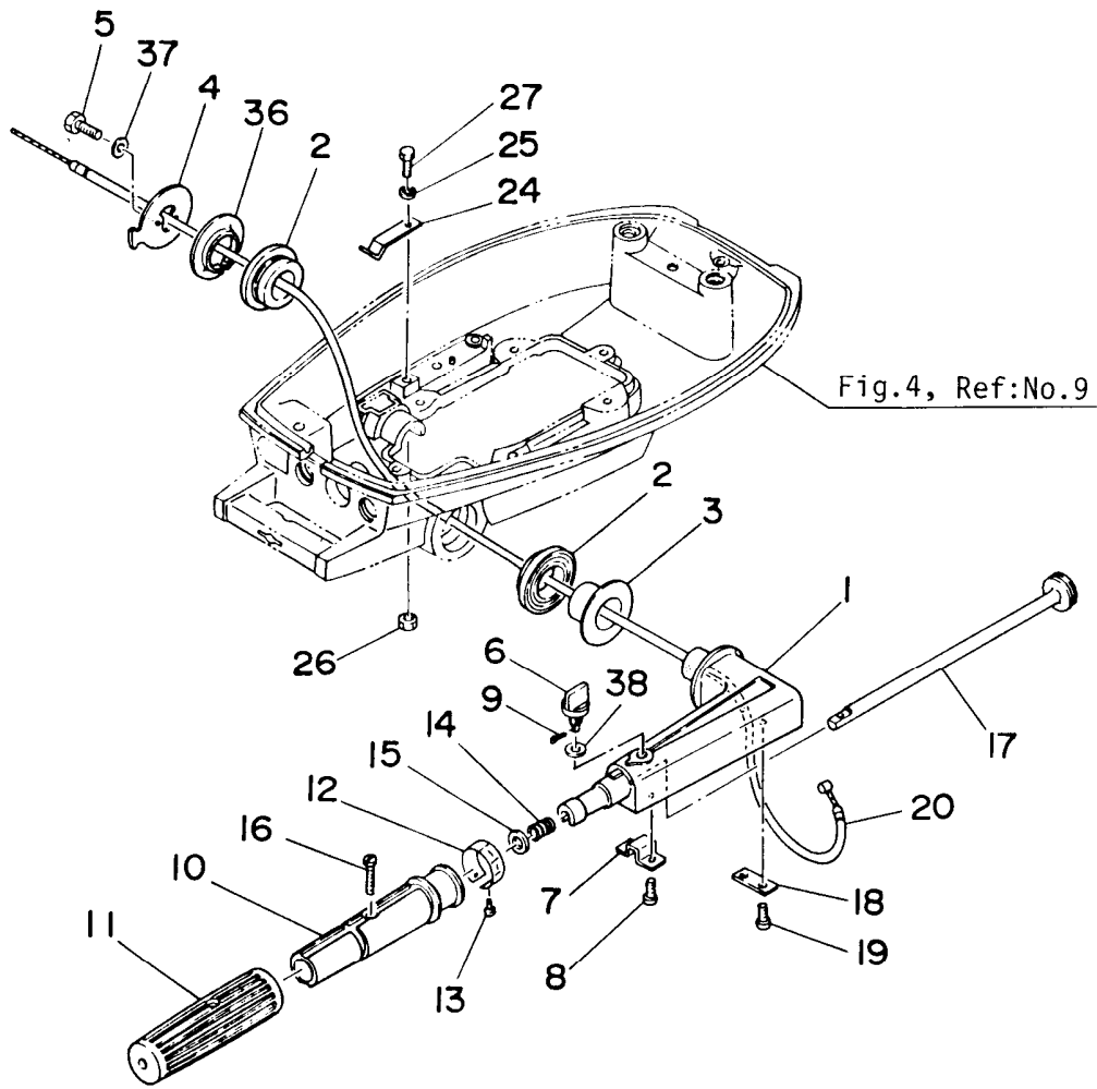
Fig. 6 CONTROL
