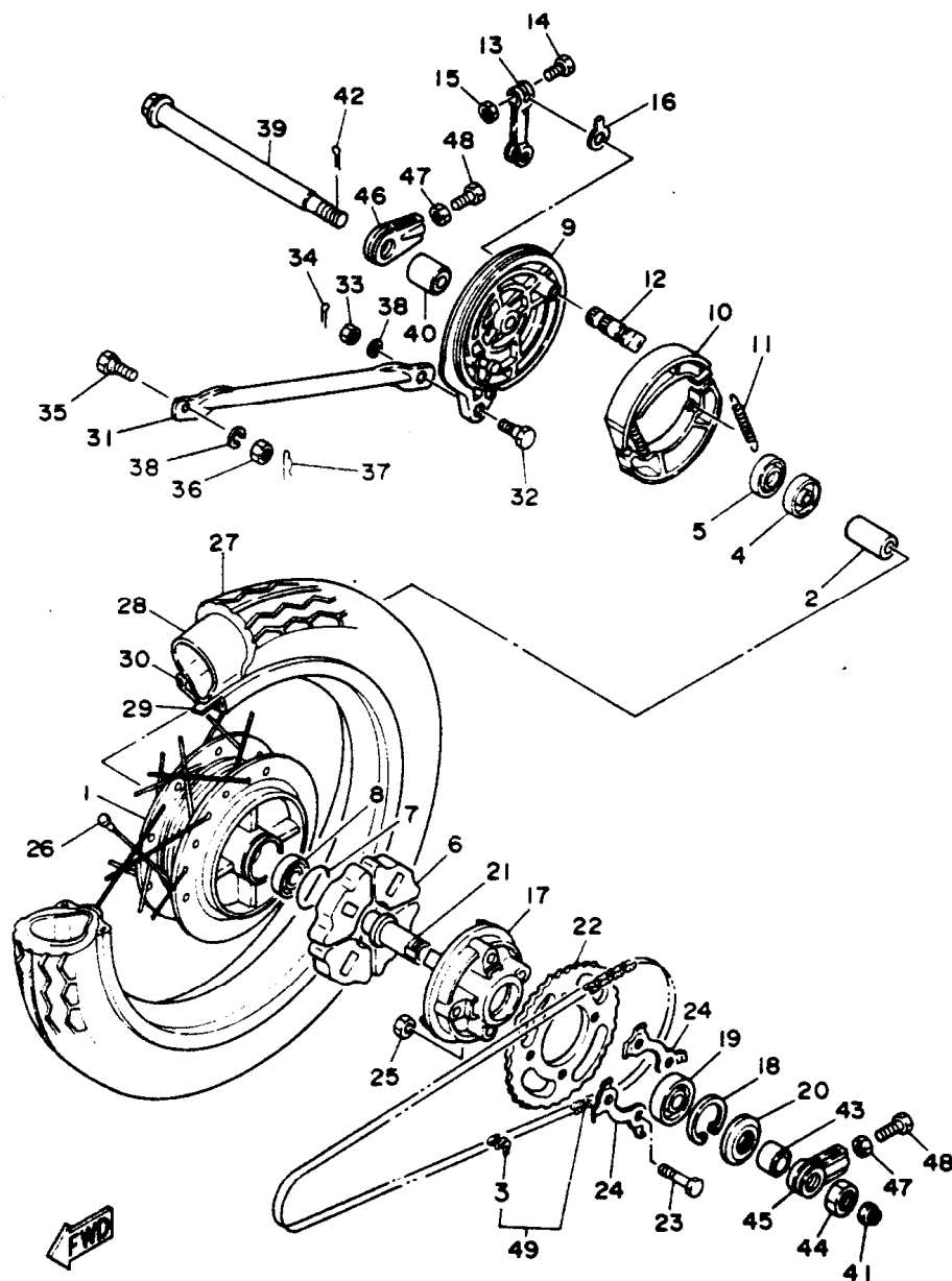
FIG. 25 – RODA TRASEIRA
