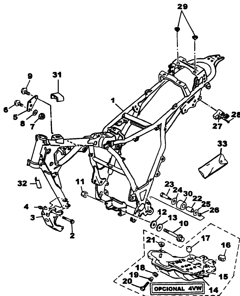
FIG. 17 - CHASSIS
