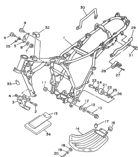
FIG.17 CHASSIS P.33 e 34
