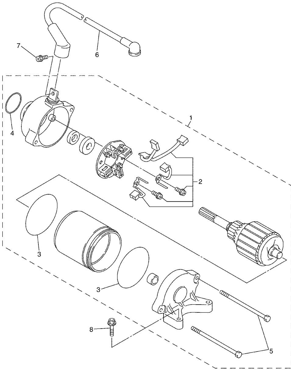
FIG. 40 STARTING MOTOR
