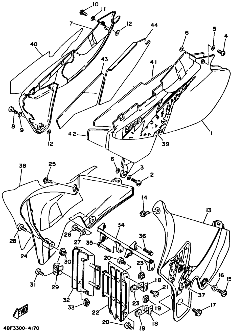
FIG. 17 SIDE COVER
