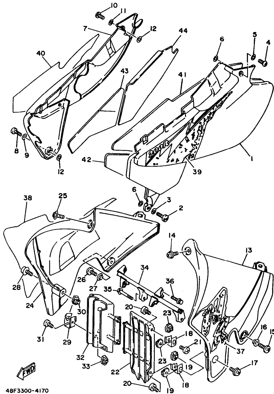
FIG. 17 SIDE COVER
