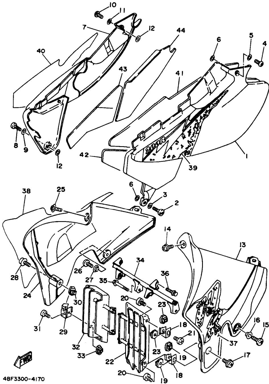
FIG. 17 SIDE COVER
