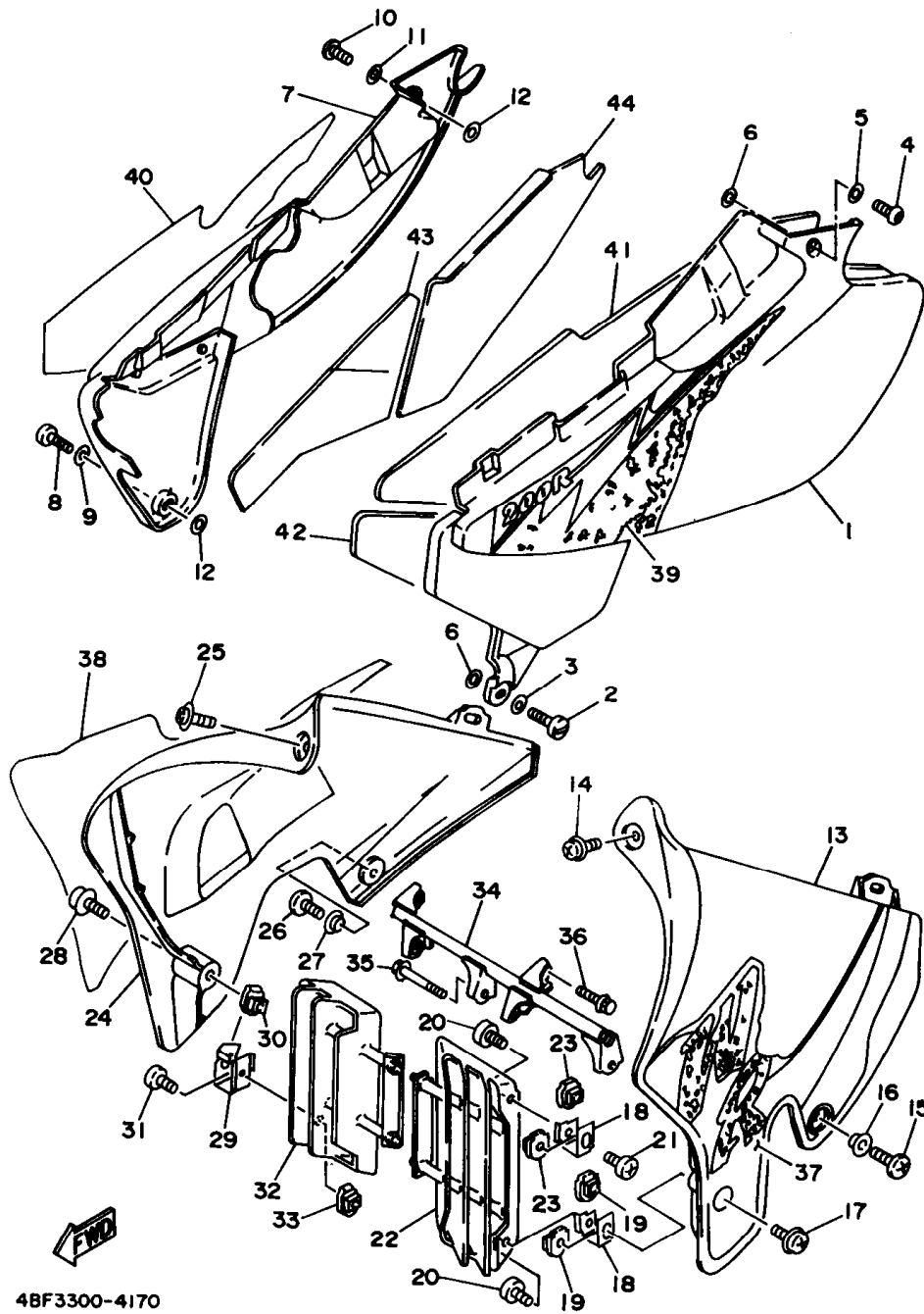
FIG. 17 SIDE COVER
