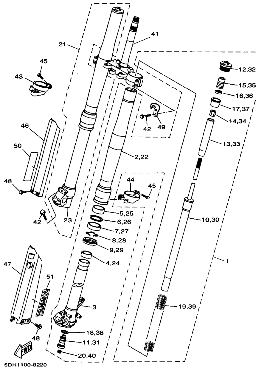
FIG. 22 FRONT FORK
